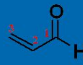
2-Propenal (Acrolein)
