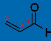
2-Propenal (Acrolein)
